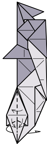
45. Fold the top layers back down, incorporating the outside reverse fold in the top layer.
